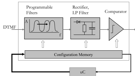
Fig. 3: Dual-tone multi-frequency decoder using adaptive filter implemented in an FPAA
