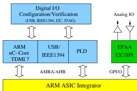
Fig. 1: RDK – Rapid Development Kit for mixed-signal systems
