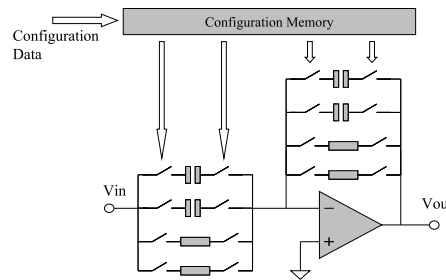
Fig. 2: Principle of programmable analog arrays
