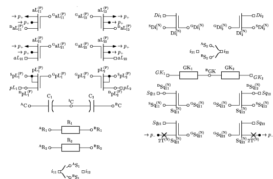
Fig. 5: EPAA: N-Cell Primitives
