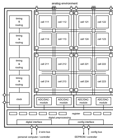
Fig. 4: EPAA - Architecture. Two buses (high- and low- speed) for configuration and data exchange
