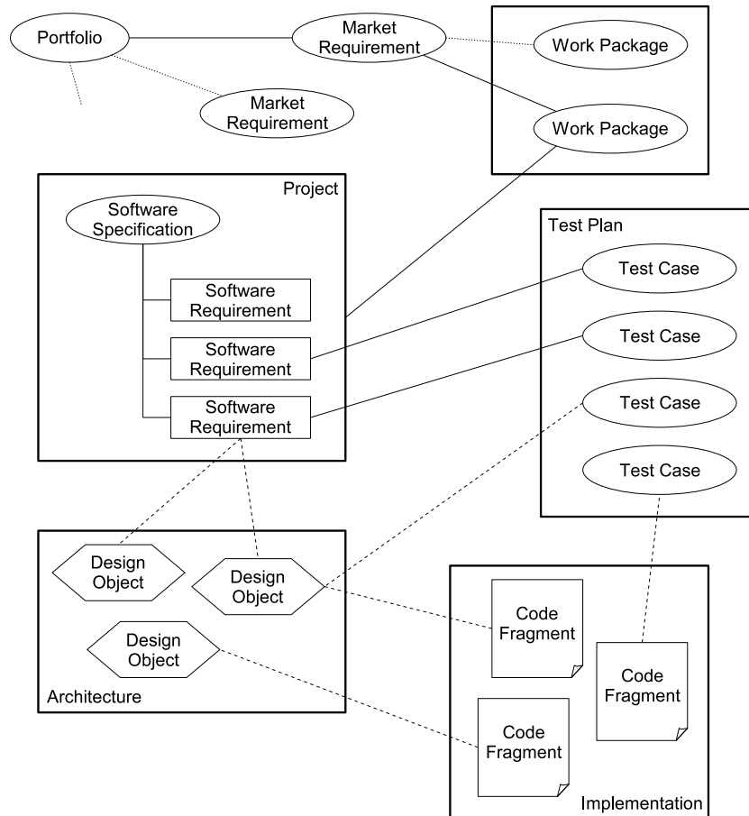
Fig. 2. Linking of Artifacts in the Development Process
